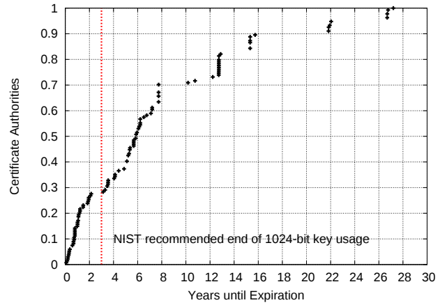
Figure 5: Expiration of 1024-bit Root Certificates —This figure shows when trusted 1024-bit RSA CA certificates expire. We note that more than 70% expire after 2016 when NIST recommends discontinuing the use of 1024-bit keys.
